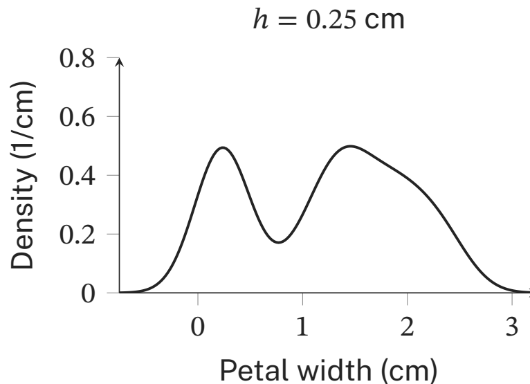
Figure 7. Petal-width Gaussian KDE with bandwidth 0.25 cm and a common evaluation grid. The curve is normalized over the full real line; the figure displays the stated finite range.
