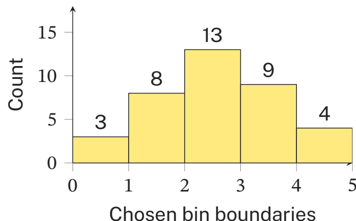
Figure 3. Five equal-width bins with counts 3, 8, 13, 9, and 4. Bar heights are calculated directly from their labelled counts.
