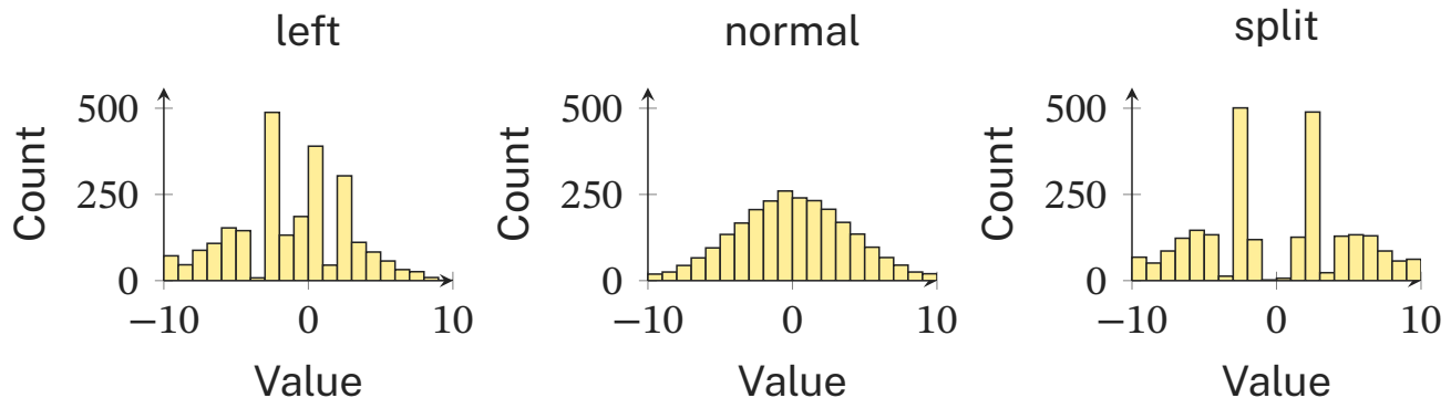
Figure 5. Source datasets named left, normal, and split, drawn from the actual observations with one shared histogram grid. The names identify the source sets; they are not diagnoses inferred from a box plot.
