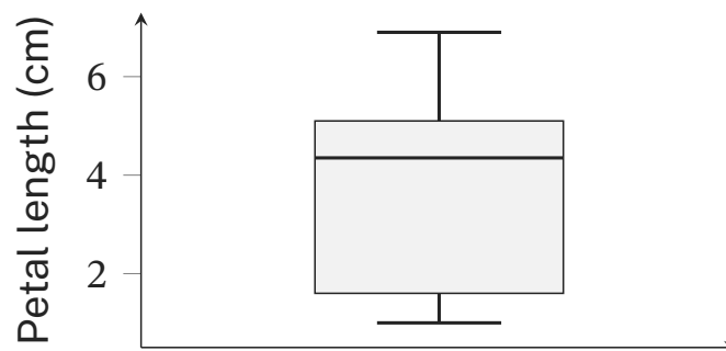
Figure 2. Petal-length box plot using linearly interpolated quartiles and the 1.5-IQR whisker rule. All plotted values are in centimetres.
