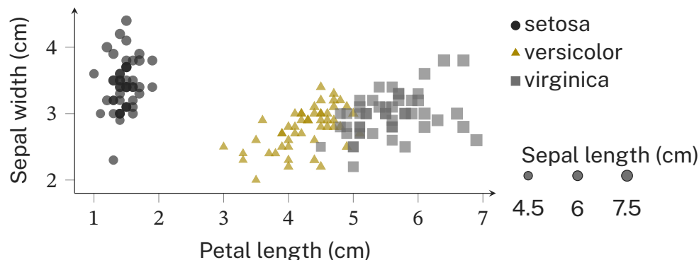
Figure 21. Petal length, sepal width, species, and sepal length in one scatter plot. The circular size key is in centimetres; proportional area comparisons apply within one marker shape.
